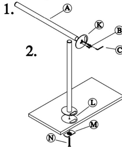
OPTION B./ Through Desk
